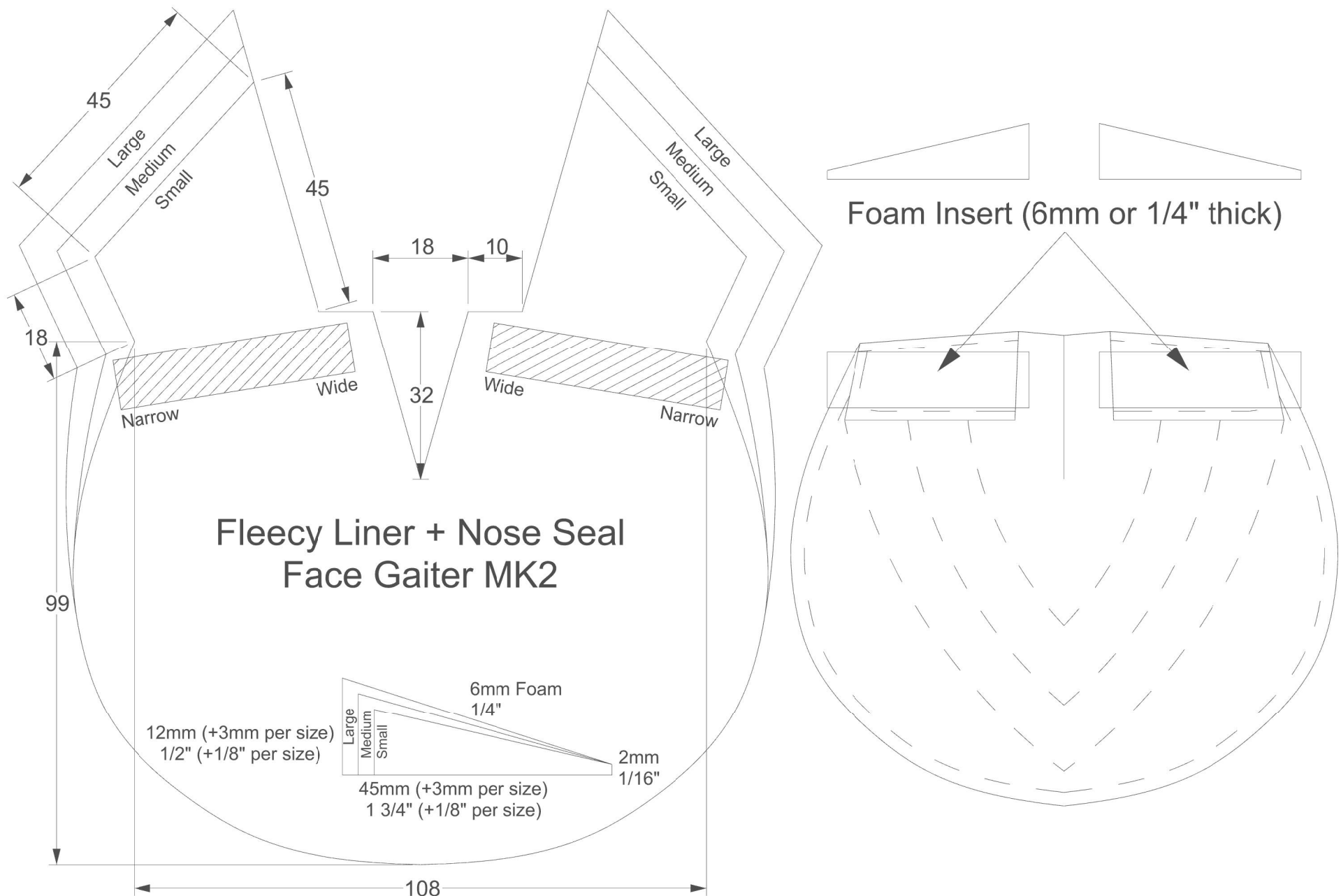
Assembly of fleece liner for MK2 Face gaiter Prints at 1:1 on Letter paper (with no margins) #MadeByBritain www.facegaiter.org
